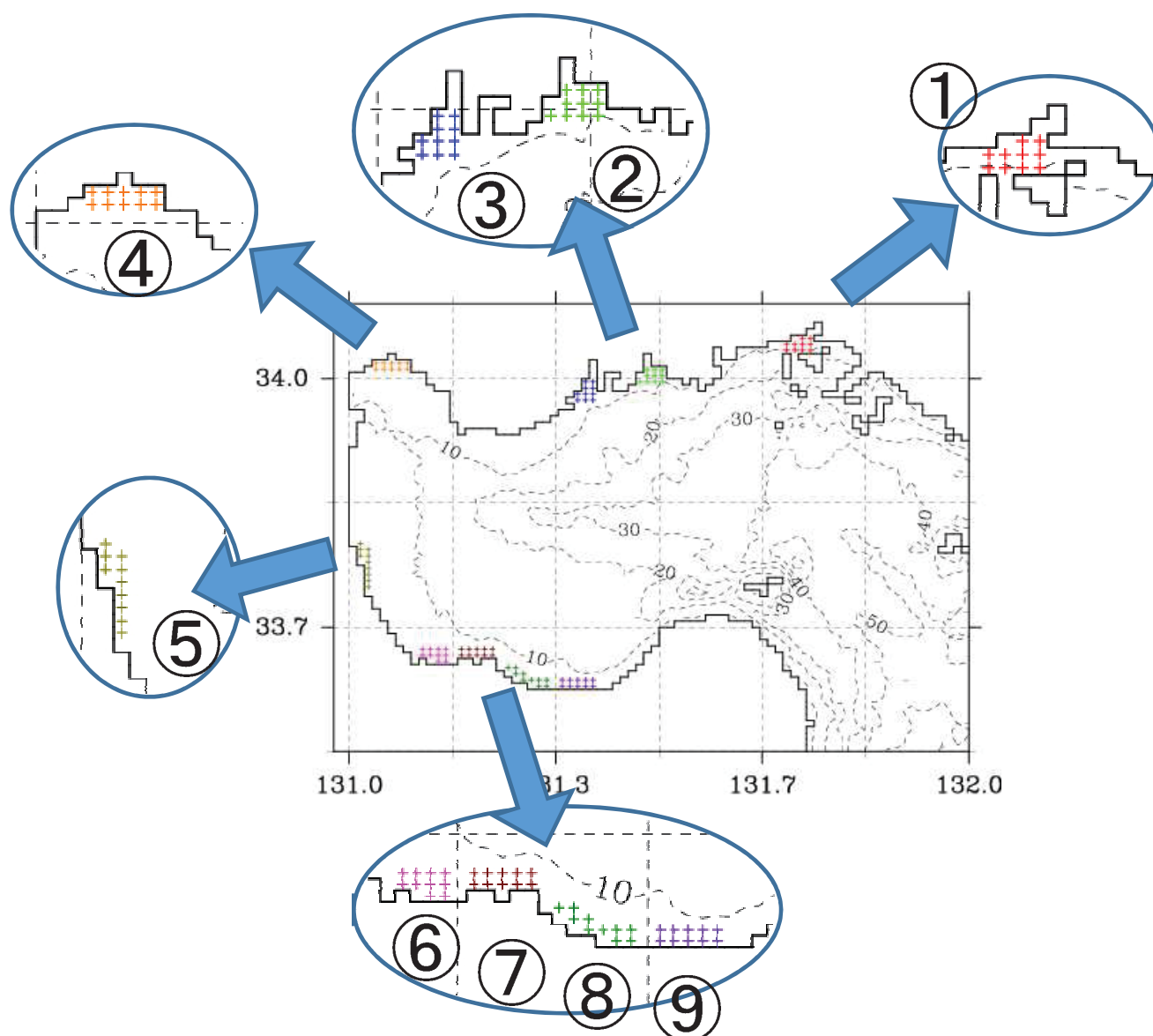
Fig. 2 Modelled larval particles were set in 9 areas along the Suo-Nada Sea coast for numerical simulation of Ruditapes philippinarum larval transport. A total of 1000 modeled larval particles were set on 10-model grids in each area. The model grids in each area were indicated as “+” symbols with identical colour.
